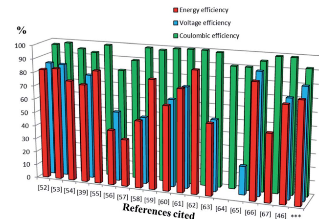
Fig. 7 The bars represent the CE, EE and VE of redox flow battery systems containing iron in their electrolyte system reported in the literature. Sequence of references followed by electrolyte system with concentration of active redox species, cell voltage (V) and volumetric capacity ( \text{Ah L}^{-1} ) are as follows: 52 1.5 \text{ M Fe}^{3+}/\text{Fe}^{2+}/1.5 \text{ M V}^{3+}/\text{V}^{2+} (1.02 V, 18 \text{ A h L}^{-1} ), 53 0.1 \text{ M Fc1N112-TFSI}/\text{Fe}(\text{acac})_3 (1.34 V, 2.47 \text{ A h L}^{-1} ), 54 \text{Fe}_3\text{O}_4/\text{Fe}/0.2 \text{ M Fe}(\text{CN})_6^{3-}/\text{Fe}(\text{CN})_6^{4-} (1.2 V, 0.00065 \text{ A h L}^{-1} ), 39 0.2 \text{ M } [\text{Fe}(\text{TEOA})\text{OH}]^{-}/[\text{Fe}(\text{TEOA})\text{OH}]^{2-}/0.2 \text{ M Fe}(\text{CN})_6^{3-}/\text{Fe}(\text{CN})_6^{4-} (1.34 V, 4 \text{ A h L}^{-1} ), 55 0.5 \text{ M 2,6-DHAQ dipotassium salt}/0.4 \text{ M K}_4\text{Fe}(\text{CN})_6 (1.20 V), 56 0.1 \text{ M FeSO}_4 + 0.5 \text{ M NaCl}/0.1 \text{ M Fe}(\text{acac})_3 , 57 1.5 \text{ M Fe}^{2+}/\text{Fe}^{3+}/1.8 \text{ M Cu}^{+}/\text{Cu}^0 (0.25 V), 58 0.5 \text{ M alloxazine-COOH}/0.4 \text{ M Fe}(\text{CN})_6^{4-} (1.3 V, 24 \text{ A h L}^{-1} ), 59 0.3 \text{ M 2,7-AQDS}/0.1 \text{ M Fe}(\text{CN})_6^{4-} (0.76 V, 17.8 \text{ A h L}^{-1} ), 60 0.5 \text{ M ACA}/0.4 \text{ M Fe}(\text{CN})_6^{4-} + 40 \text{ mM Fe}(\text{CN})_6^{3-} (1.13 V), 61 0.5 \text{ M } (\text{NH}_4)_4[\text{Fe}(\text{CN})_6]/0.5 \text{ M } (\text{SPR})_2\text{V} (0.82 V, 10 \text{ A h L}^{-1} ), 62 0.1 \text{ M bislawson}/0.2 \text{ M K}_4\text{Fe}(\text{CN})_6/0.02 \text{ M K}_3\text{Fe}(\text{CN})_6 (1.05 V), 63 0.1 \text{ M Cr}(\text{acac})_3/0.1 \text{ M Fe}(\text{acac}) (1.2 V, 0.67 \text{ A h L}^{-1} ), 64 0.01 \text{ M Co}(\text{phen})_3/0.01 \text{ M Fe}(\text{phen})_3 (2.1 V, 0.10 \text{ A h L}^{-1} ), 65 0.2 \text{ M } [\text{Co}(\text{bpy})_3]\text{Tf}_2/0.2 \text{ M } [\text{Fe}(\text{bpy})_3]\text{Tf}_2 (2.0 V), 66 0.1 \text{ M FeCp}_2\text{PF}_6/0.1 \text{ M CoCp}_2 (1.7 V, 2.5 \text{ A h L}^{-1} ), 67 0.20 \text{ M K}_4\text{Fe}(\text{CN})_6 , 0.08 \text{ M K}_3\text{Fe}(\text{CN})_6/0.1 \text{ M 2,6-DBEAQ} (1.05 V), 46 0.5 \text{ M Co(II)-mTEA}/0.25 \text{ M Fe(III)-TEA} + 0.5 \text{ M Fe(II)-TEA} (0.93 V) and ***this work.
