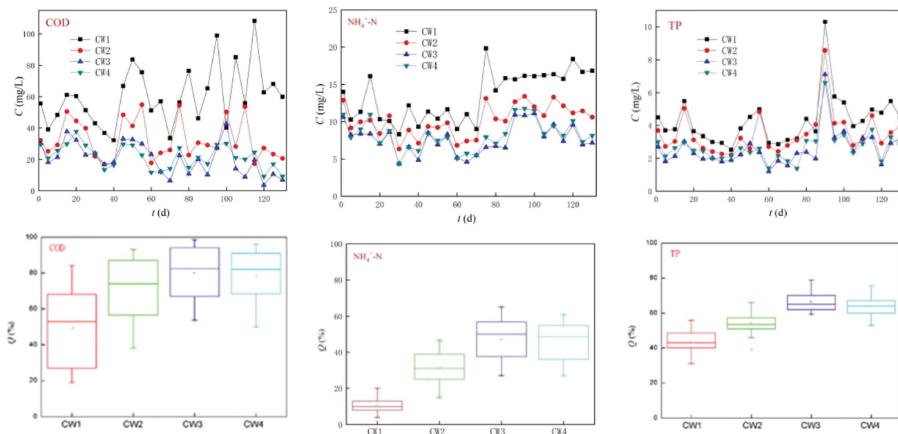
Fig. 7 Removal effect of four constructed wetlands on conventional pollutants.
