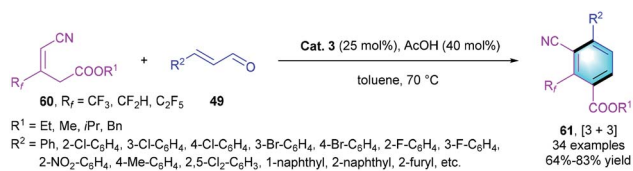
Plausible mechanism for the [3 + 3] benzannulation
