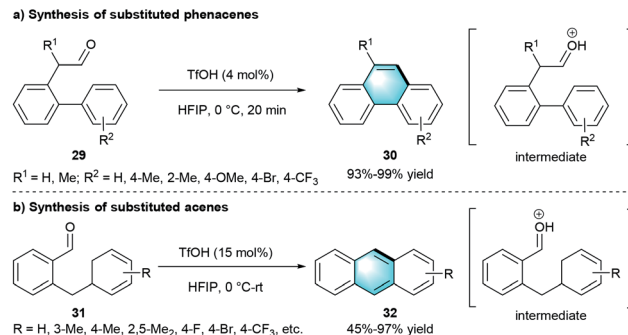
Scheme 8 TfOH-catalyzed intramolecular benzannulation to synthesize phenacenes and acenes.
