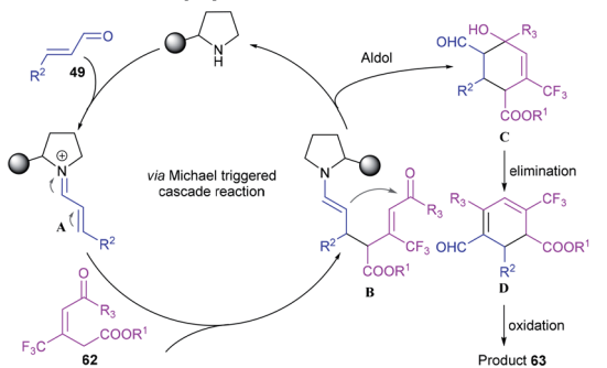
c) Synthesis of biaryls through RC-type reaction
