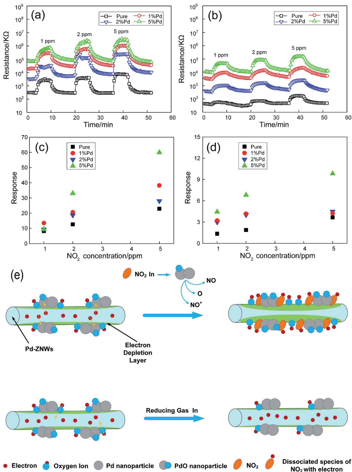
Fig. 3 Dynamic responses of the sensors based on pure ( @150^\circ C ) and Pd-ZNWs ( @100^\circ C ) upon exposure to NO_2 gas with various concentrations at (a) 30% RH and (b) 60% RH. The corresponding sensor responses as a function of NO_2 concentration at (c) 30% RH and (d) 60% RH. (e) Sensing mechanisms of Pd-ZNWs towards NO_2 and reducing gas. This figure has been reproduced with permission from ref. 91, Elsevier, Copyright 2019 (License Number: 4923990843354).
