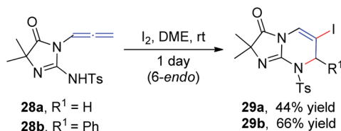
Scheme 10 Iodine-mediated intramolecular cyclization of 3-allenyl-1-imidazolinones.
