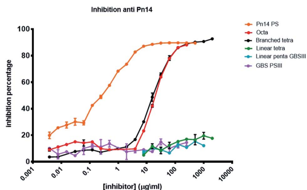
Fig. 3 Inhibition percentage of Sp14 capsular polysaccharide using a specific murine serum (saccharide concentration expressed as \mu\text{g mL}^{-1} ).
