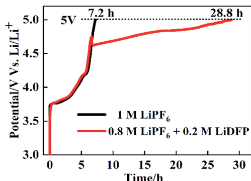
Fig. 9 The overcharge protection performance of NCM811/Li cells with different electrolytes.
