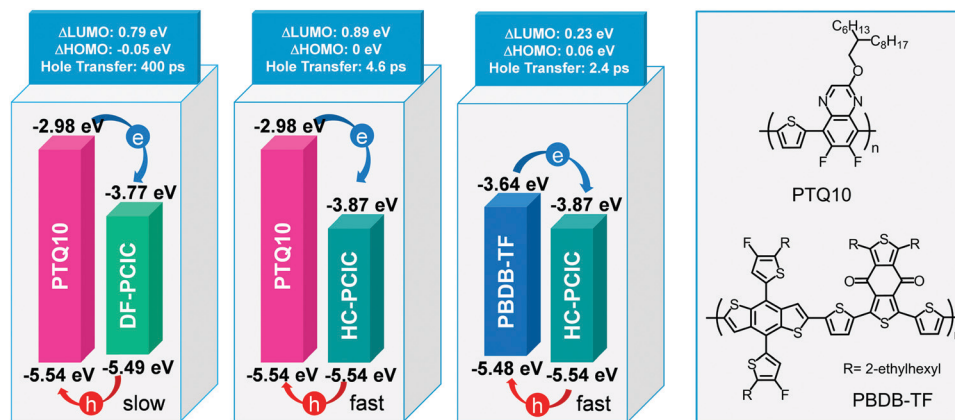
Fig. 30 Diagram of hole transfer for different blends with various HOMO offsets and hole transfer rates. Adapted from ref. 217 with permission. Copyright (2019) American Chemical Society.
