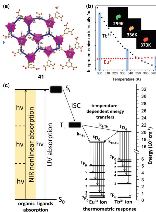
Fig. 33 (a) Honeycomb-like Eu/Tb mixed 2D coordination polymer 41 . (b) Plots of the integrated intensity of ^5D_0 \rightarrow ^7F_2 of Eu(III) (red dots) and ^5D_4 \rightarrow ^7F_5 of Tb(III) (black dots) f-f emission as a function of temperature (excited at 337 nm). Insets: Photographs showing the emission color of 41 at 299, 336, and 373 K, respectively. (c) Energy level diagram highlighting the use of three-photon excitation for effecting the thermometric luminescent response. Reprinted with permission from ref. 145. Copyright 2019 American Chemical Society.
