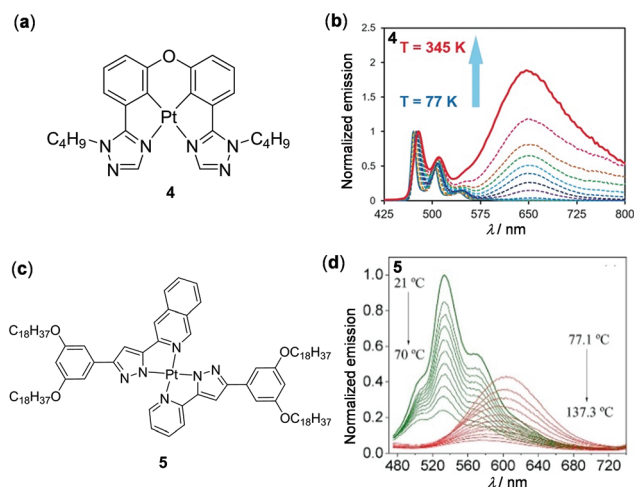
Fig. 4 (a) Molecular structure of Pt(II) complex 4 . (b) Normalized temperature-dependent emission spectra of 4 in degassed Me-THF ( 1 \times 10^{-3} \text{ M} , \lambda_{\text{ex}} = 397 \text{ nm} ). Reprinted with permission from ref. 91. Copyright 2017 Wiley-VCH. (c) Molecular structure of Pt(II) complex 5 . (d) Normalized temperature-dependent emission spectral changes of the PMMA film doped with 5 upon heating from 21 to 137.3^\circ\text{C} . Reprinted with permission from ref. 92. Copyright 2020 Elsevier Ltd.
