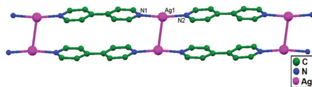
Fig. 32 The 1D molecular ladder made of [\text{Ag}(4,4'\text{-bpy})]_n sides and ligand-unsupported \text{Ag-Ag} interactions in 54.
