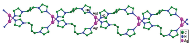
Fig. 30 The formation of a double-helical chain via ligand-unsupported \text{Ag-Ag} interactions in 50.
