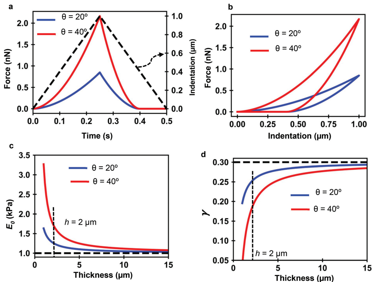
Fig. 7 PLR simulations for two conical tips. (a) Force-time curves. The dashed line shows the waveform of the indentation. Conical tips of half-angles 20^\circ (blue) and 40^\circ (red); h = 2\ \mu\text{m} . Tip velocity of 4\ \mu\text{m s}^{-1} . (b) Corresponding force-distance curves. (c) Apparent elastic modulus value as a function of the thickness. (d) Apparent power-law exponent dependence on the thickness. The apparent PLR parameters have been determined by fitting the FDCs generated with the analytical finite-thickness theory (eqn (7) and (12)) with the expressions describing a semi-infinite material (eqn (13)).
