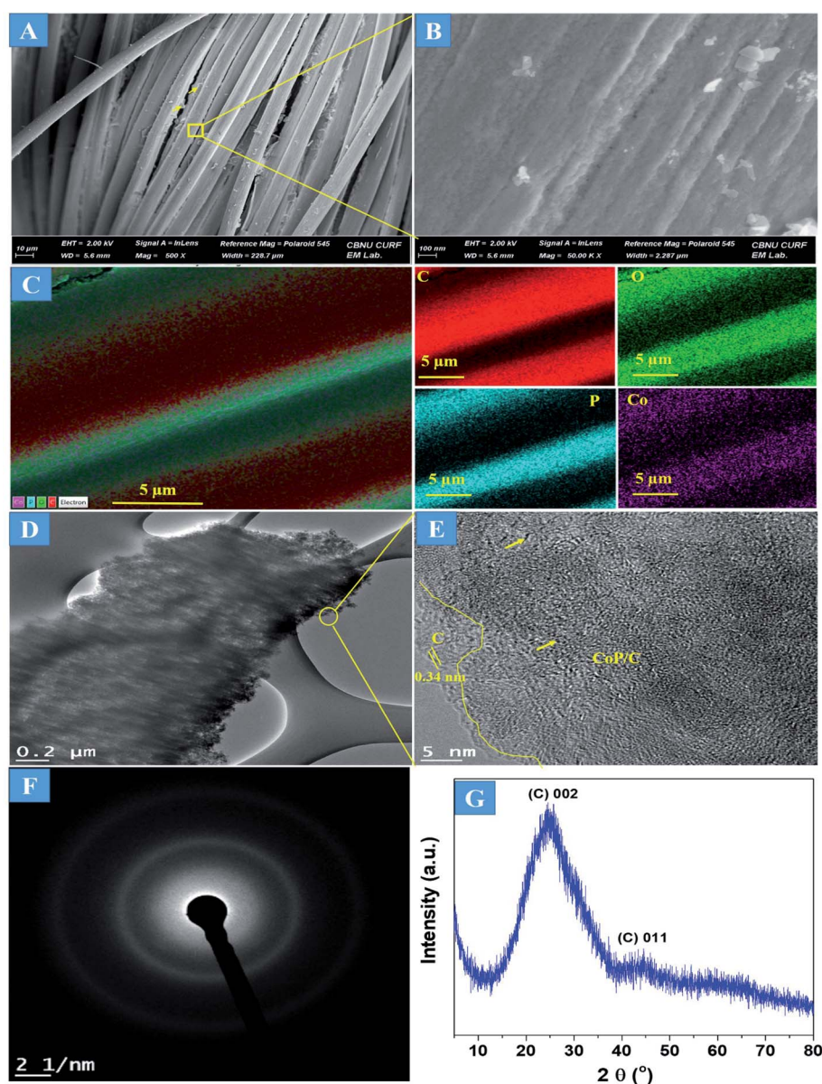
Fig. 1 FE-SEM images (A and B), elemental mapping images (C), HRTEM images (D and E), SAED pattern (F), and (G) XRD spectrum of the a-PC@CoPi-CC8.
