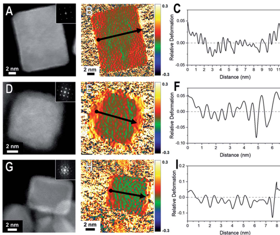
Fig. 2 HAADF-STEM images and corresponding GPA for the thin (2–4 ML) shelled samples (A–C) Pd@Pt, (D–F) Rh@Pd, and (G–I) Rh@Pt nanocrystals. The first column consists of the HAADF-STEM images of the nanocrystal examined by GPA. The second column contains the corresponding GPA colors maps which correspond to the in-plane strain ( \epsilon_{xx} ) field (which is the strain in the plane of the crystal face) where the intensity scale shows relative deformation. The third column contains line profiles of the lattice difference determined by GPA with the line profile locations indicated by arrow in the GPA color maps where the start of the line profile begins at the dot and ends at the arrow head.
