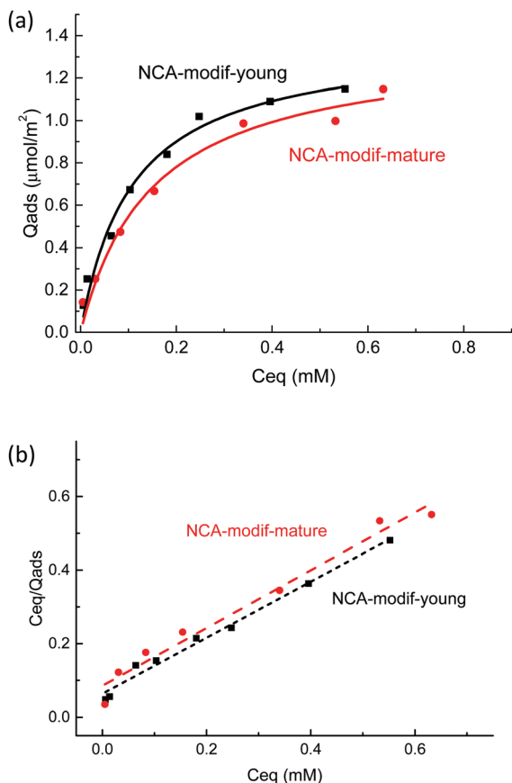
Fig. 7 (a) \text{U}(\text{vi}) adsorption isotherms by NCA-modif-young, NCA-modif-mature and HA-ref and (b) linear regression of NCA-modif-young and NCA-modif-mature using Langmuir isotherm models.
