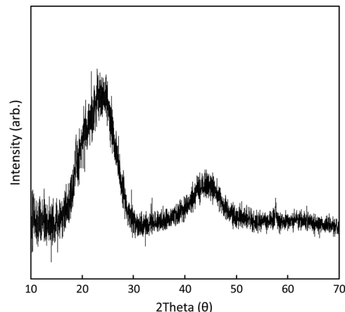
Fig. 4 PXRD pattern of 1C .
