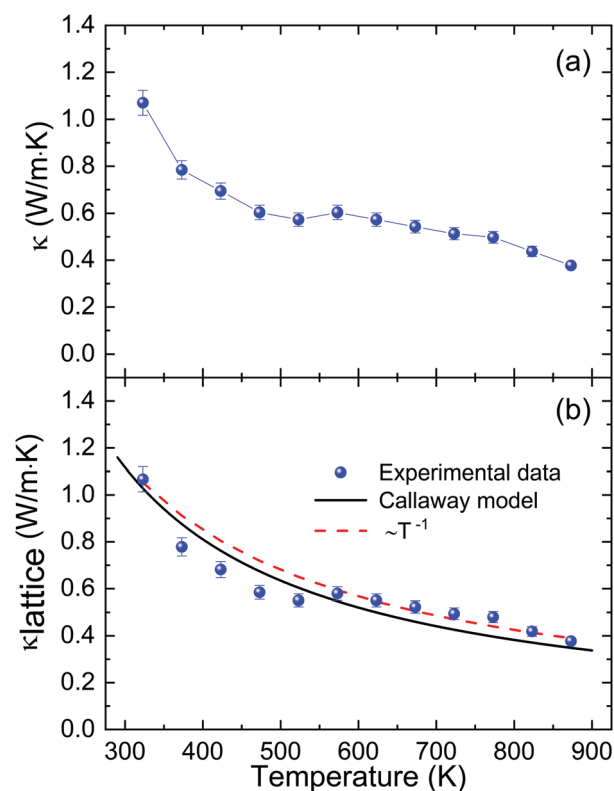
Fig. 10 Temperature dependence of the (a) total thermal conductivity and (b) lattice thermal conductivity of microwave-synthesized \text{Sn}_{1-\delta}\text{S} . The black solid line represents the data calculated using the Callaway model, 76 while the dotted line shows the \sim T^{-1} fit.
