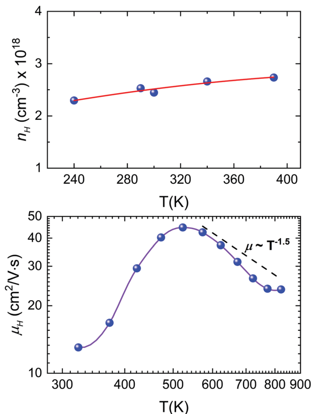
Fig. 8 (a) Temperature dependence of the Hall carrier concentration ( n_H ). (b) Temperature dependence of the Hall carrier mobility ( \mu_H ) of \text{Sn}_{1-\delta}\text{S} . The Hall carrier density of \sim 2.5 \times 10^{18} \text{ cm}^{-3} measured at room temperature is assumed to be unchanged up to 823 K. The solid lines are a guide to the eye. The dotted line corresponds to the \mu \sim T^{-1.5} temperature dependence.
