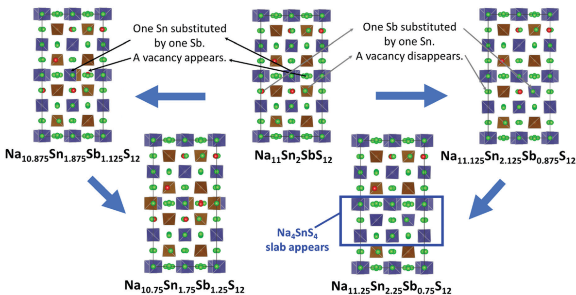
Fig. 4 Schematic representation of derivation of the \text{Na}_{9+x}\text{Sn}_x\text{Sb}_{3-x}\text{S}_{12} structures with x = 1.75, 1.875, 2.125 and x = 2.25 . Blue (brown) tetrahedra represent SnS 4 (SbS 4 ), green spheres occupied Na sites. Na vacancies are marked in red. For \text{Na}_{11.25}\text{Sn}_{2.25}\text{Sb}_{0.75}\text{S}_{12} the lowest energy structure contains a slab of \text{Na}_4\text{SnS}_4 composition marked in blue.
