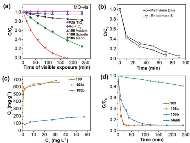
Fig. 22 (a) Comparative photocatalytic degradation of MO of commercial \text{TiO}_2 , \text{Ag-TiO}_2 , polymer nanofibers of 105 , vesicles and nanospindles of polymer 106 under visible light ( \text{P25-TiO}_2 is \text{TiO}_2 with a diameter of 25 nm). (b) Photocatalytic degradation of RhB and MB using polymer 107 . (c) The adsorption isotherms of RhB for polymers 108a , 108b and 109 at 25 °C. (d) Removal of RhB with polymers 108a , 108b and 109 in the supernatant. Reprinted with permission from ref. 215–217. Copyright 2015 Nature Publishing Group, 2015 Wiley-VCH and 2015 Royal Society of Chemistry.
