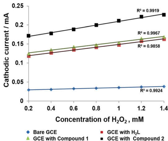
Fig. 7 Relationship between cathodic current and \text{H}_2\text{O}_2 concentration in the four cases mentioned above (Fig. 5).
