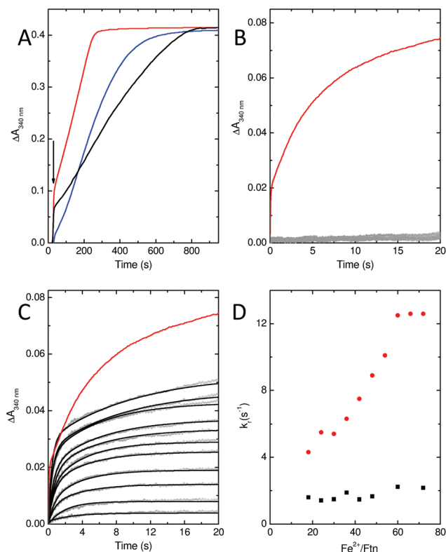
Fig. 4 Iron oxidation kinetics of SynFtn variants D137A and E62A. (A) Mineral core formation following the addition of 200 \mu\text{M Fe}^{2+} to 0.5 \mu\text{M SynFtn} variant E62A (black trace) or D137A (blue trace). Red trace shows the response of the wild type protein for comparison. (B) Iron oxidation following rapid mixing of 1 \mu\text{M D137A SynFtn} with an equal volume of 6\text{--}96 \mu\text{M Fe}^{2+} . (C) As (B) but for SynFtn variant E62A. Black traces in panel C represent bi-exponential fits to the data. In panels B and C, data points are shown as gray circles, red traces represent the response of wild type protein upon mixing with 96 \mu\text{M Fe}^{2+} for comparison. (D) Apparent rate constant of the rapid phase extracted from exponential fits shown in panel (C) (black squares) together with the equivalent data reported for the wild type protein (red circles) for comparison. All measurements were conducted at pH 6.5 and 25^\circ\text{C} .
