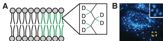
Fig. 6 SRS lipid imaging. (A) Deuterated palmitate and oleate incorporated into lipid acyl chains. (B) SRS imaging of C–D single bond stretches in cells treated with palmitate-d 31 reveals patches of slow lateral diffusion in the ER [adapted with permission from Y. Shen, Z. Zhao, L. Zhang, L. Shi, S. Shahriar, R. B. Chan, G. Di Paolo and W. Min, Proc. Natl. Acad. Sci. U. S. A. , 2017, 114 , 13394–13399]. 26
