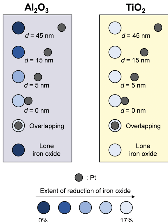
Fig. 8 Spillover on \text{Al}_2\text{O}_3 and \text{TiO}_2 traced using Pt-iron oxide pairs.
