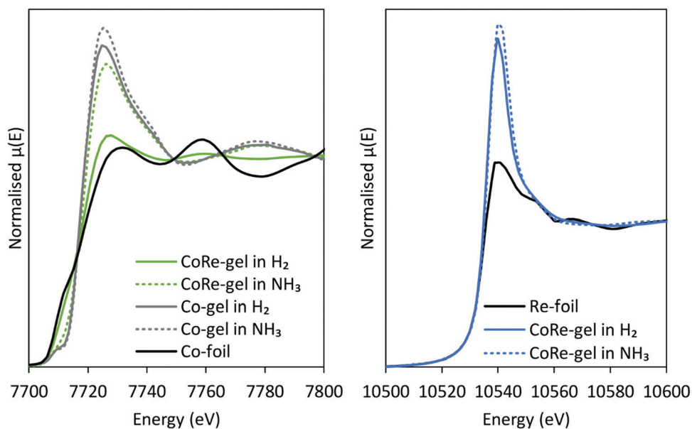
Fig. 9 XANES-spectra before and after switching from \text{H}_2 to \text{NH}_3 from the Co K-edge (left) and Re \text{L}_{\text{III}} -edge (right).
