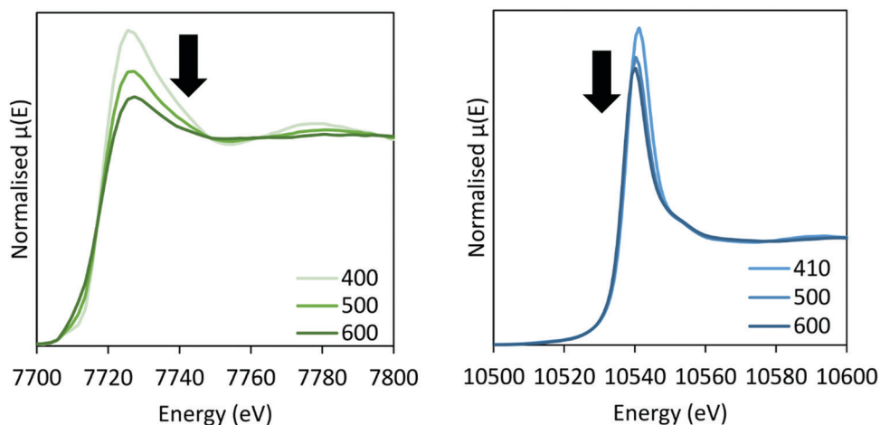
Fig. 11 XANES of the CoRe-gel during ammonia decomposition at the Co K-edge (left) and Re \text{L}_{\text{III}} -edge (right) between 400\text{--}600^\circ\text{C} in 5% \text{NH}_3 .
