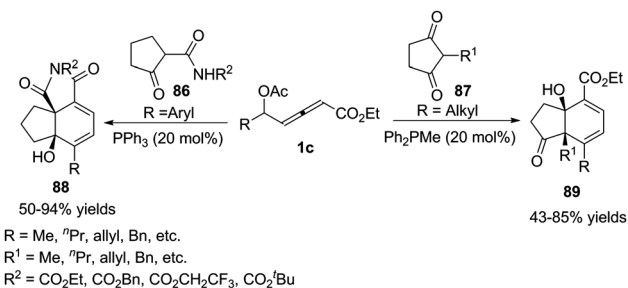
Scheme 28 Phosphine-catalysed (4+2) annulations of \delta -acetoxy allenates and ketones. 50-94% yields R = Me, n Pr, allyl, Bn, etc. R 1 = Me, n Pr, allyl, Bn, etc. R 2 = CO 2 Et, CO 2 Bn, CO 2 CH 2 CF 3 , CO 2 t Bu 1,3-dipole intermediate
