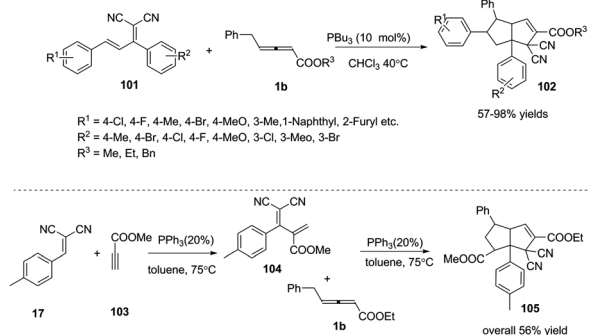
Scheme 32 Phosphine-catalysed sequential (2+3) and (3+2) annulation reactions of \gamma -substituted allenones with conjugate dienes.
