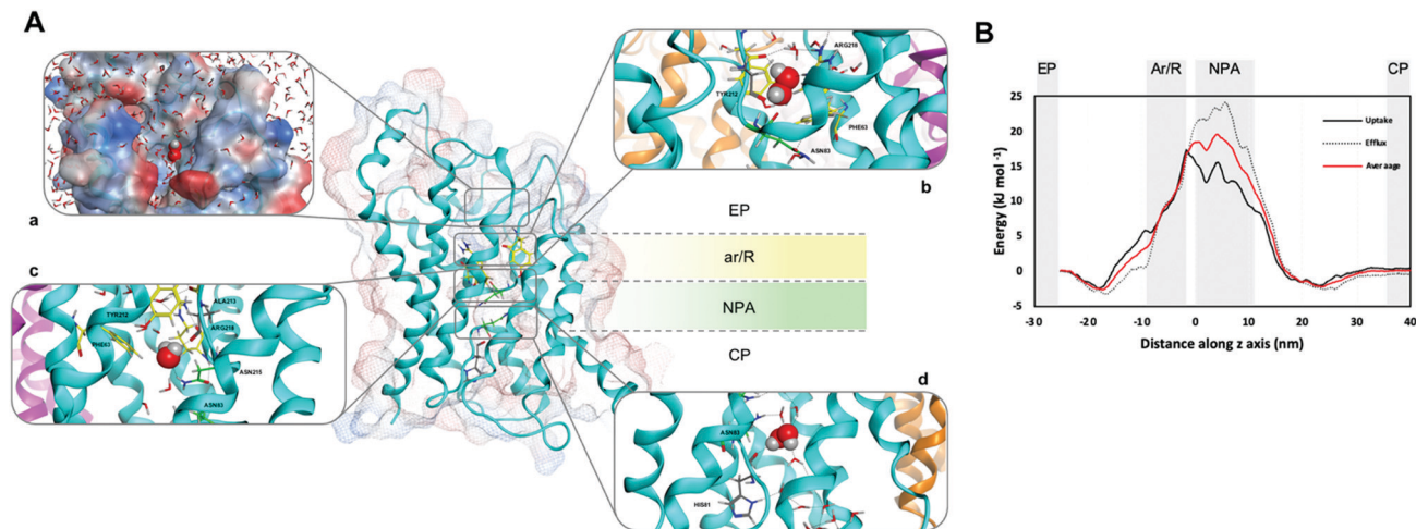
Fig. 1 (A) hAQP3 monomer showing the ar/R (yellow) and NPA (green) selectivity filters. (a) Position of \text{H}_2\text{O}_2 as it enters the extracellular pocket of hAQP3 with lipophilic/hydrophilic molecular surface (hydrophilic = blue, lipophilic = red). (b) \text{H}_2\text{O}_2 orientation within the ar/R SF including H-bond network with residues Tyr212, Ala213 and Arg218. (c) \text{H}_2\text{O}_2 orientation during translocation between ar/R and NPA selectivity filters, interacting with residues Ala213 and Asn215 of the NPA motif. (d) \text{H}_2\text{O}_2 orientation when leaving the NPA selectivity filter, including H-bond network involving His81 and a bridging water molecule to Asn83. Figure generated using the MOE software. 23 (B) Average free-energy surface of \text{H}_2\text{O}_2 uptake (solid line) and efflux (dashed line), calculated using metadynamics sampling. Averaged curve shown in red.
