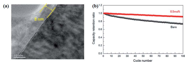
Fig. 14 (a) TEM image of a cross section of a 0.5 mol% LZO coated NCA particle. The right hand (dark) side corresponds to NCA; (b) cycle characteristics of bare and 0.5 mol% LZO coated NCA at 25 °C. Reproduced with permission. 121 Copyright© 2013, Elsevier B.V.
