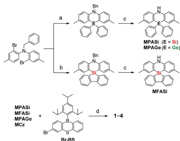
Scheme 1 Synthetic schemes for 1–4. Reagents and conditions: (a) (i) n -BuLi, Et 2 O, 0 °C, 1 h, (ii) Ph 2 EtCl 2 (E = Si, Ge), 35 °C, 2 h; (b) (i) n -BuLi, Et 2 O, 0 °C, 1 h, (ii) 5,5-dichlorodibenzo[ b,d ]silole, 35 °C, 2 h; (c) H 2 , Pd/C, CH 2 Cl 2 /AcOH, RT, 15–24 h; (d) Pd 2 (dba) 3 , t -Bu 3 PH·BF 4 , NaOt-Bu, toluene, 100 °C, 6–17 h. Bn = benzyl, MCz = 1,3,6,8-tetramethylcarbazole.
