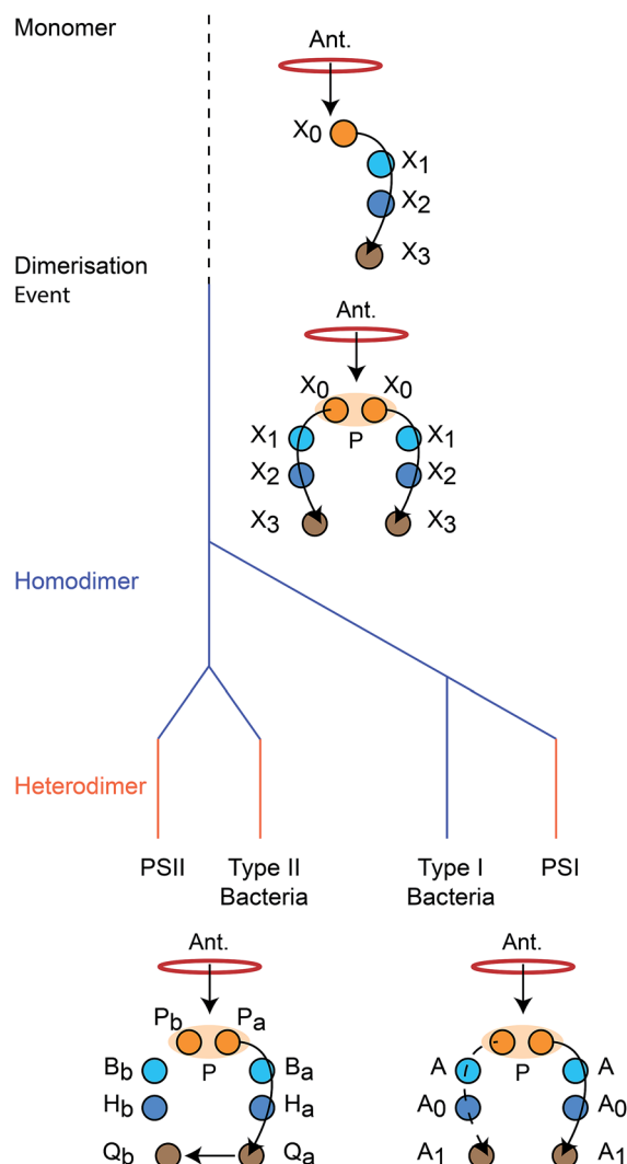
Fig. 2 Evolution of reaction centres (RC). 1 The primordial RC was monomeric, likely comprising three BChls (X 0 , X 1 , X 2 ) and a quinone (X 3 ). An antenna (Ant.) would transfer an exciton to X 0 , which would also serve as the charge donor. The charge would transfer through X 1 and X 2 before arriving at X 3 . The monomeric RC dimerised, producing a homodimer with two identical copies of the monomer, connected at the special pair (P). Excitons from the antenna could delocalise over P before charge separation, with charge transfer occurring along either branch. The homodimer subsequently diverged into type I and type II RCs, some of which experienced gene duplication events that led to heterodimerism. In modern type I RCs, each branch consists of three (B)Chls (P, A, and A 0 ) and a quinone (A 1 ). In heterodimeric PSI, charge transfer occurs exclusively down one branch, while in homodimeric systems (such as heliobacteria) charge can move down either branch with equal probability. In modern type II RCs, each branch consists of two (B)Chls (P and B), a phaeophytin (H) and a quinone (Q). Charge travels down one branch before being transferred to the inactive-branch quinone.
