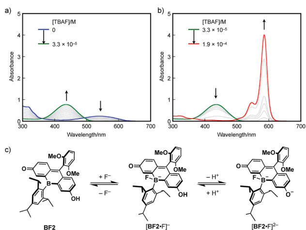
Fig. 5 UV-vis absorption spectral changes of BF2 in acetonitrile ( 2.8 \times 10^{-5} M) upon addition of TBAF: (a) [\text{TBAF}]/[\text{BF2}] = 0 to 3.3 \times 10^{-5} and (b) 3.3 \times 10^{-5} to 1.9 \times 10^{-4} . (c) Equilibrium between neutral BF2 , borate [\text{BF2} \cdot \text{F}]^- , and borate fluorescein anion [\text{BF2} \cdot \text{F}]^{2-} .
