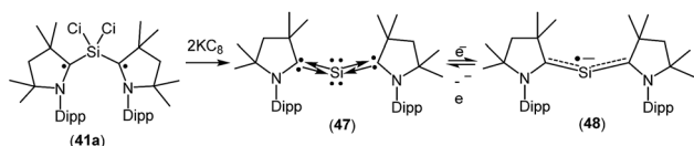
Fig. 13 cAAC-stabilized siladicalcarbene and in situ generation of ( Me2 cAAC) 2 Si •− .
