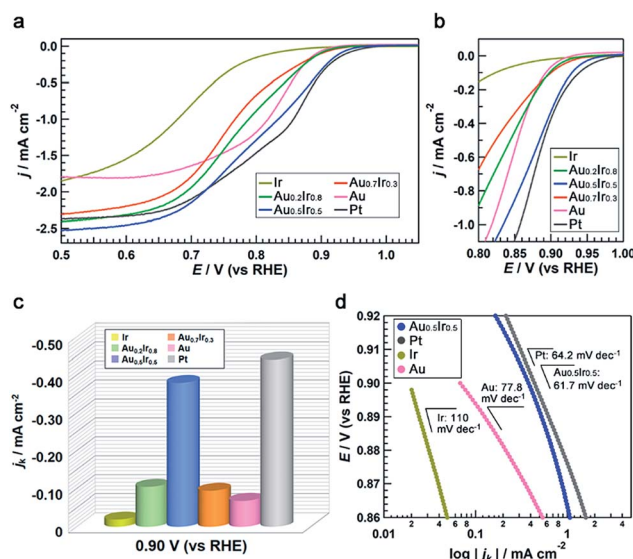
Fig. 5 Electrochemical oxygen-reduction activities of \text{Au}_x\text{Ir}_{1-x} alloy catalysts. (a), (b) rotating disk electrode I - V polarization curves taken in \text{O}_2 -saturated 1.0 M NaOH aqueous solution normalized by the glassy carbon electrode geometric area ( 0.196 \text{ cm}^2 ) (a) from 0.50 to 1.05 \text{V}_{\text{RHE}} and (b) from 0.80 to 1.00 \text{V}_{\text{RHE}} . (c) Summary of the kinetic current densities for oxygen reduction on each catalyst measured at 0.90 \text{ V}_{\text{RHE}} . (d) Tafel plots for the catalysts. All of the NPs were loaded on carbon support.
