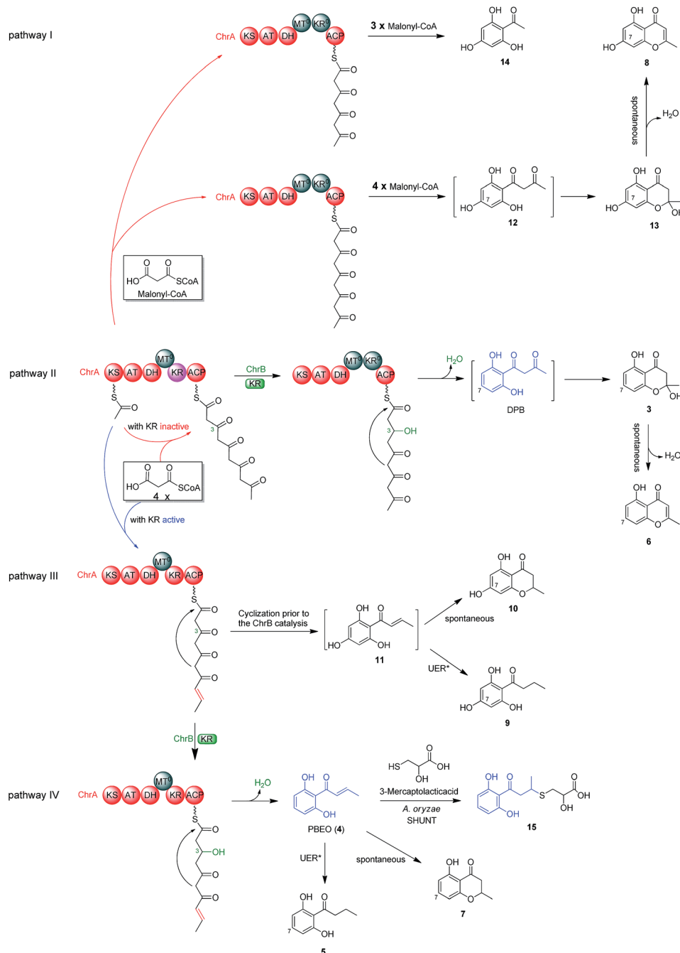
Fig. 4 Metabolic network of polyketides encoded by the chrA gene cluster in D. eschscholzii . ChrA is a partially reducing polyketide synthase (PR-PKS) with the domains of \beta -ketoacylsynthase (KS), acyltransferase (AT), dehydratase (DH), C-methyltransferase (MT 0 , inactive), ketoreductase (KR, active/inactive) and acyl carrier protein (ACP). ChrB is a ketoreductase partner that catalyzes the selective 3-ketone reduction of acyclic pentaketide with acetonyl or allyl side-chain terminals. UER*, unspecific enoyl reductase expressible in D. eschscholzii and A. oryzae .
