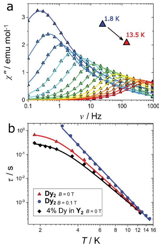
Fig. 5 (a) Experimental (triangles) and fitted (solid lines) frequency dependence of the imaginary component of the magnetic susceptibility ( \chi'' ) at B = 0 \text{ T} . (b) Relaxation times (symbols) extracted from \chi'' fit at various temperatures and for \text{Dy}_2 at B = 0 \text{ T} (red triangles) and at B = 0.1 \text{ T} (blue dots) and for 4% Dy diluted in \text{Y}_2 (black diamonds). Lines represent the best fits (see text).
