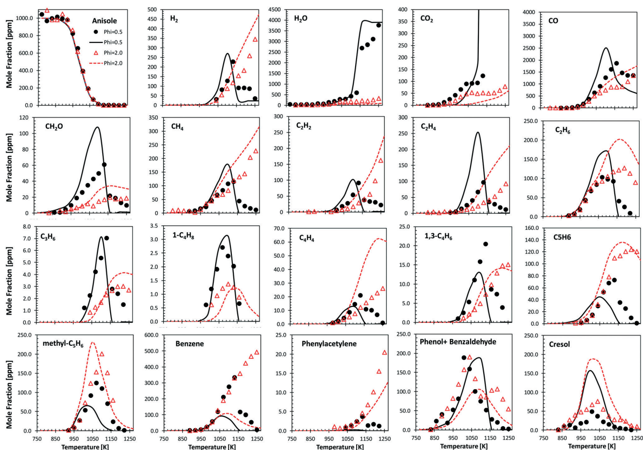
Fig. 9 Anisole atmospheric pressure oxidation in an Orleans JSR. 75 0.1% anisole/ \text{O}_2/\text{N}_2 mixtures under rich ( \varphi = 2.0 , triangles) and lean conditions ( \varphi = 0.5 , circles). Comparisons between experimental data (symbols) and model predictions (lines).
