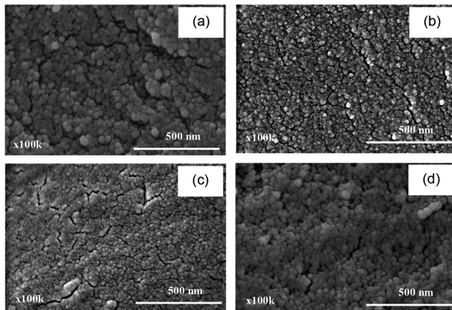
Fig. 5 PEDOT:PSS surface morphology at the EDOT : \text{Na}_2\text{S}_2\text{O}_8 mole ratio of 1 : 1 and at various EDOT : PSS weight ratios: EDOT : PSS weight ratio of (a) 1 : 1, (b) 1 : 5, (c) 1 : 11 and (d) 1 : 13.
