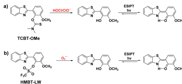
Scheme 1 (a) Our previously reported ESIPT probe for the detection of HOCl/CLO - . (b) This work – a trifluoromethanesulfonate linker-based ESIPT HMBT-LW for the detection of O 2 •- .
