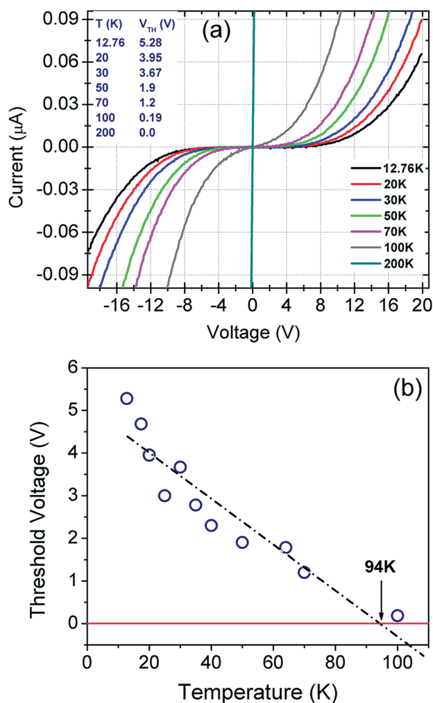
Fig. 4 (a) Temperature dependent I - V plots of the sensor in the bias range from -20 V to +20 V. (b) Threshold voltage ( V_{\text{TH}} ) as a function of temperature.
