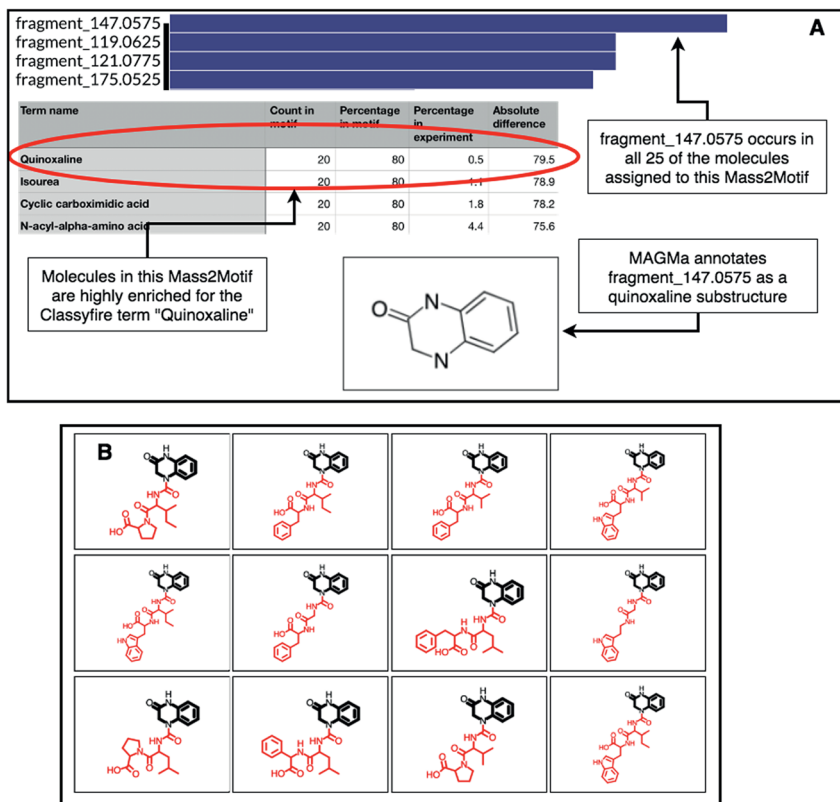
Fig. 4 (A) Top: feature frequency plot for GNPS Mass2Motif 60; middle: most enriched ClassyFire substituent terms in the same motif; bottom: MAGMa assigned the quinoxalino substructure in 22 of the 25 molecules associated to this motif. (B) Screenshot of the ms2lda.org web app with the MAGMa annotated quinoxalino substructure highlighted in 12 of the 22 molecules.
