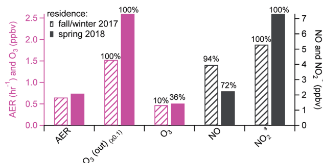
Fig. 2 Average AER, ambient outdoor O_3 levels, and mixing ratios of O_3 and nitrogen oxides in the residence under background conditions in two seasons. Data below the detection limit were included to calculate averages. Text above the bars indicates the percentage of data above the detection limit.
