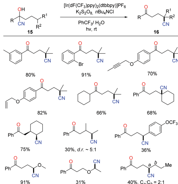
Scheme 18 Free alcohol-directed cyanation of remote C(\text{sp}^3)\text{-H} bonds.
