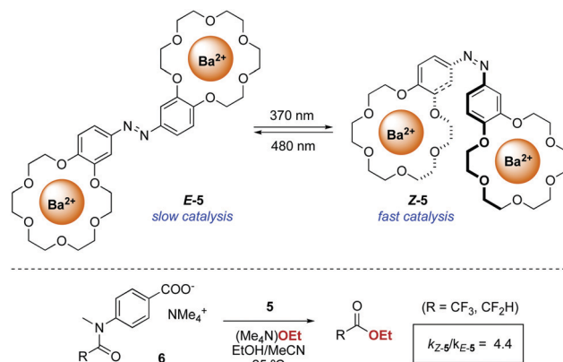
Scheme 3 Photoswitchable catalyst 5 for the ethanoylation of 6 .
