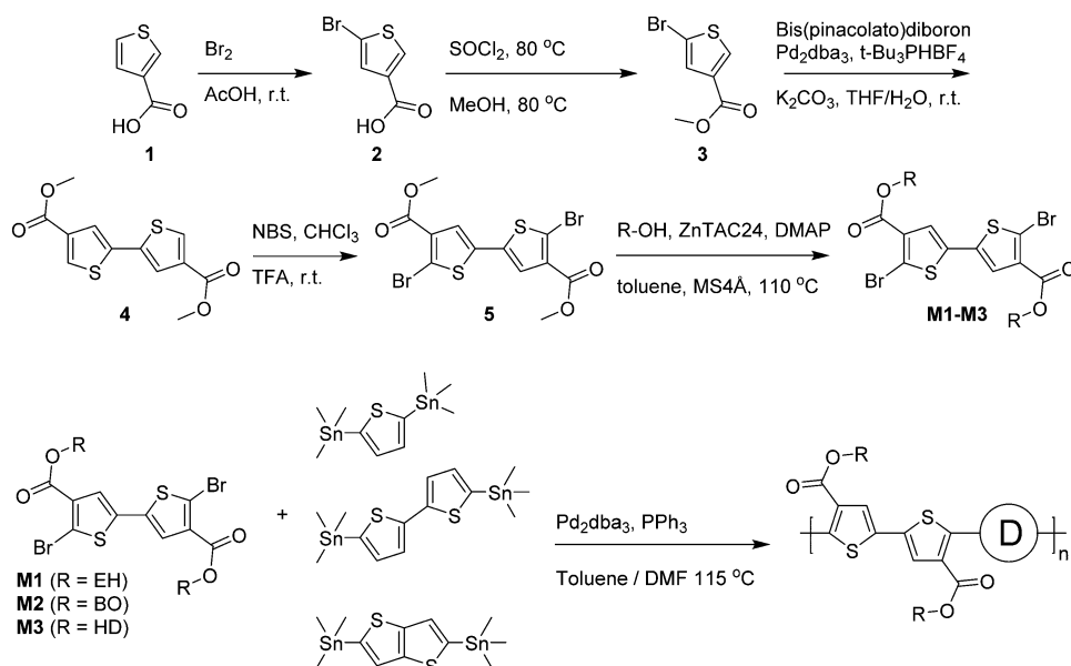
Scheme 1 Synthesis routes towards 2-ethylhexyl (EH), 2-butyloctyl (BO) and 2-hexyldodecyl (HD) substituted dicarboxylic ester bithiophene monomers (DCB) (top) and polymerization conditions for all nine combinations of monomers M1–M3 and thiophene (T), bithiophene (2T) and thienothiophene bistannyl monomers (TT) (bottom).
