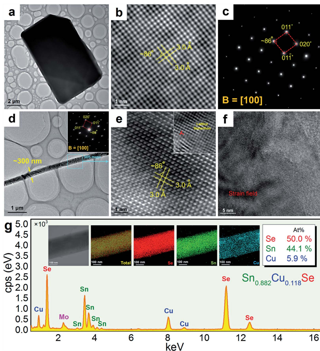
Fig. 3 (a) TEM image of a typical SnSe microplate for x = 0 , corresponding (b) HRTEM image and (c) SAED pattern taken from the plate shown in (a). (d) TEM image of a section of a typical SnSeCu microbelt for x = 0.118 , inset showing the corresponding SAED pattern, (e) corresponding HRTEM image with a dislocation shown in the inset. (f) TEM image showing significant strain contrast. (g) EDS map and spot analysis taken from a typical SnSeCu microbelt for x = 0.118 .
