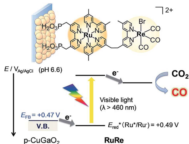
Scheme 16 Schematic illustration for the photocatalytic reduction of \text{CO}_2 to CO with the RuRe/CuGaO 2 electrode. Reprinted with permission from ref. 173. Copyright 2017, Royal Society of Chemistry.
