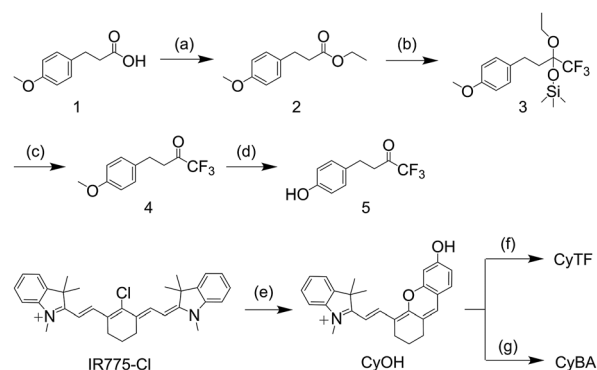
Scheme 2 Synthetic route of CyTF and CyBA . (a) H 2 SO 4 (con.), reflux, 4 h, EtOH, 97%; (b) TMSF 3 , CsF, THF, 18 h, 86%; (c) TBAF, THF, 5 h, then 4 M HCl, 3 h, 97%; (d) BBr 3 , -78 °C, room temperature, 12 h, CH 2 Cl 2 , 74%; (e) K 2 CO 3 , resorcinol, CH 3 CN, 2 h; (f) 5 , BTC, Et 3 N, 0 °C, 2 h, CH 2 Cl 2 , 28%; (g) 4-methylphenylboronic acid pinacol ester, K 2 CO 3 , CH 3 CN, 75%.
