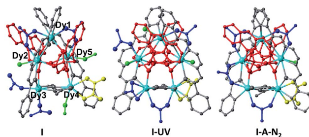
Fig. 2 The pentameric units in the structures of I, I-UV and I-A-N 2 . The common fragments (2EDDC 2- and 2 acetate) are shown in grey, Dy in cyan, other acetate in blue, C 15 H 11 PO 3 in red, oxalate in yellow, and H 2 O and CH 3 OH solvents in green.
