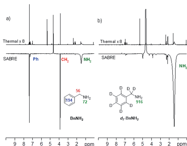
Fig. 2 (a) ^1\text{H} NMR spectra of \text{BnNH}_2 , thermally polarised, top, and hyperpolarised, bottom. (b) ^1\text{H} NMR spectra for d_7 - \text{BnNH}_2 , thermally polarised, top, and hyperpolarised, bottom.
