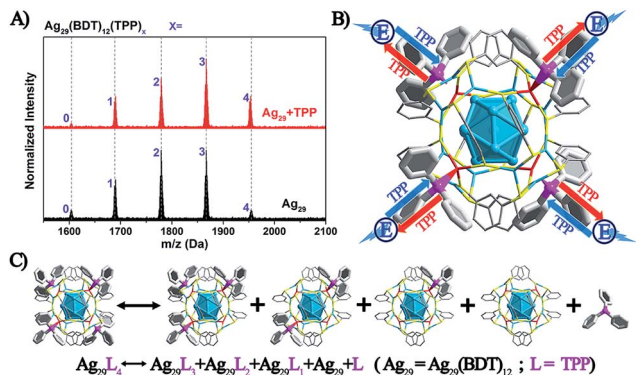
Fig. 3 (A) ESI-MS spectra of the \text{Ag}_{29}(\text{BDT})_{12}(\text{TPP})_4 NC with or without the addition of TPP. (B) Illustration of the dynamic TPP dissociation–aggregation process on the \text{Ag}_{29}(\text{BDT})_{12}(\text{TPP})_4 and the corresponding energy loss. (C) The dynamic TPP dissociation–aggregation reversible reaction. Color codes: cerulean/red spheres, Ag; yellow spheres, S; purple spheres, P; grey spheres, C; white spheres, H.
