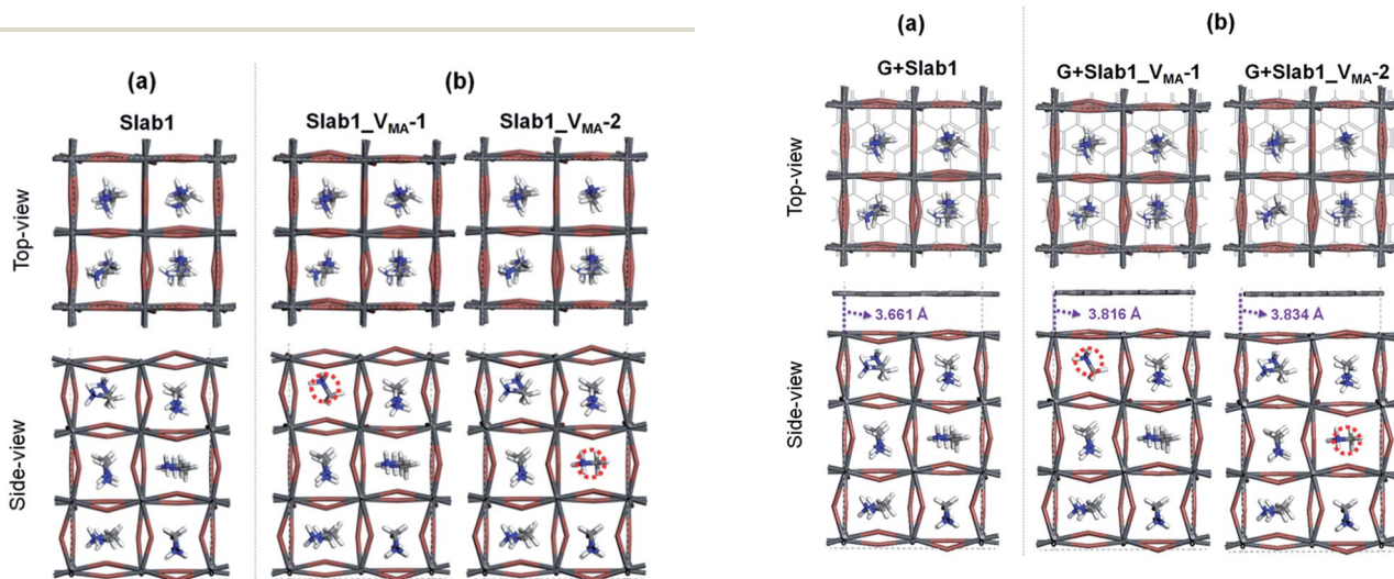
Fig. 17 (a) Defect-free and (b) V_{MA} -containing defective graphene + MAPbI_3 hybrids.
