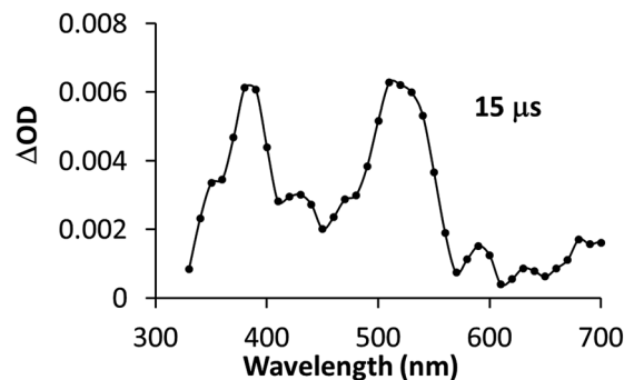
Fig. 9 Transient absorption spectrum of a solution containing \text{PS}_{\text{Ir}}^+ (50 μM), \text{Et}_3\text{N} (20 mM) and \mathbf{1}^{\text{CO2Et}} (80 μM) recorded at 15 μs after laser excitation. All measurements were carried out under \text{N}_2 at room temperature in acetonitrile ( \lambda_{\text{ex}} = 355 nm, E = 8 mJ per pulse).
